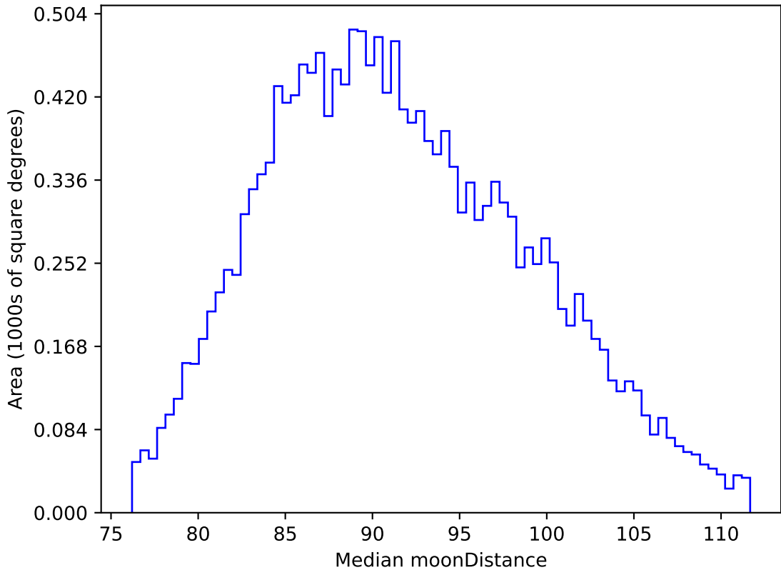
ddf_acor_sf15_lsf40_lsr10_v3.4_10yrs WFD i band: Median moonDistance
