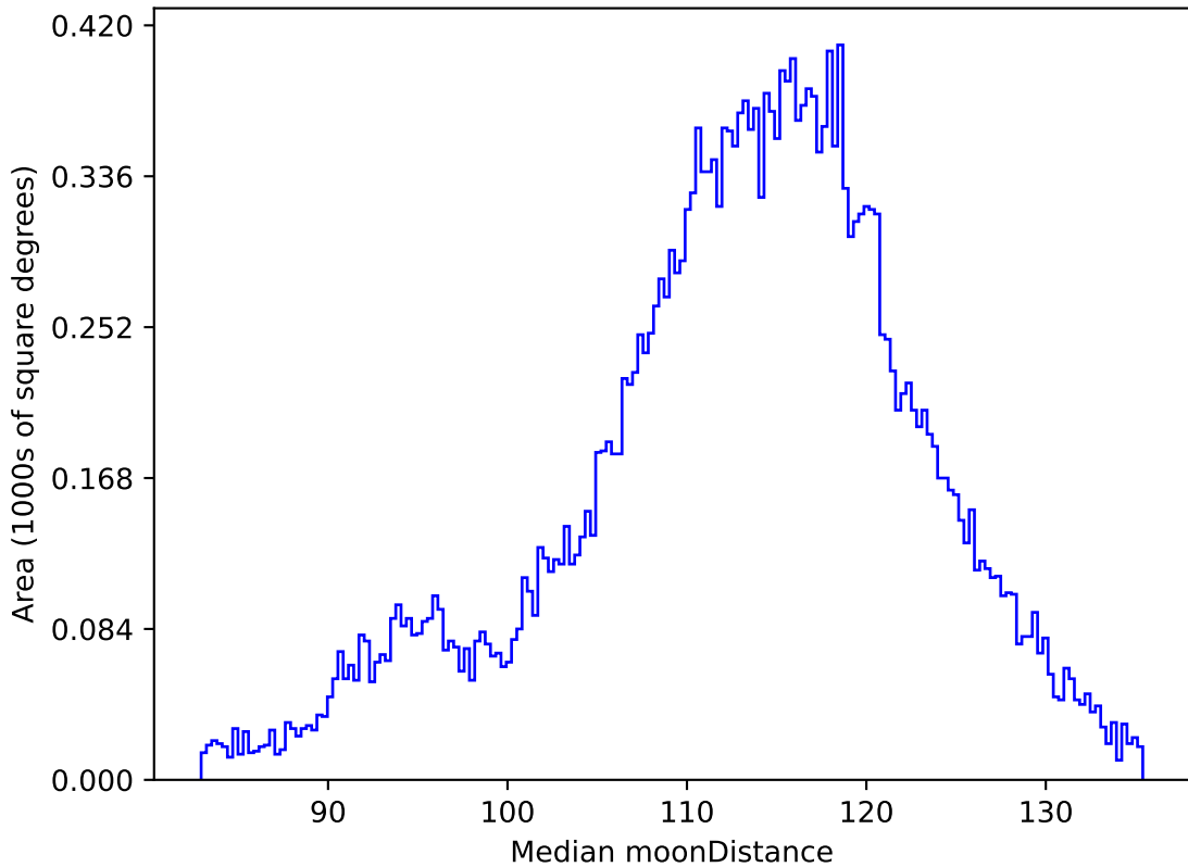
ddf_acor_sf15_lsf40_lsr10_v3.4_10yrs All sky r band: Median moonDistance
