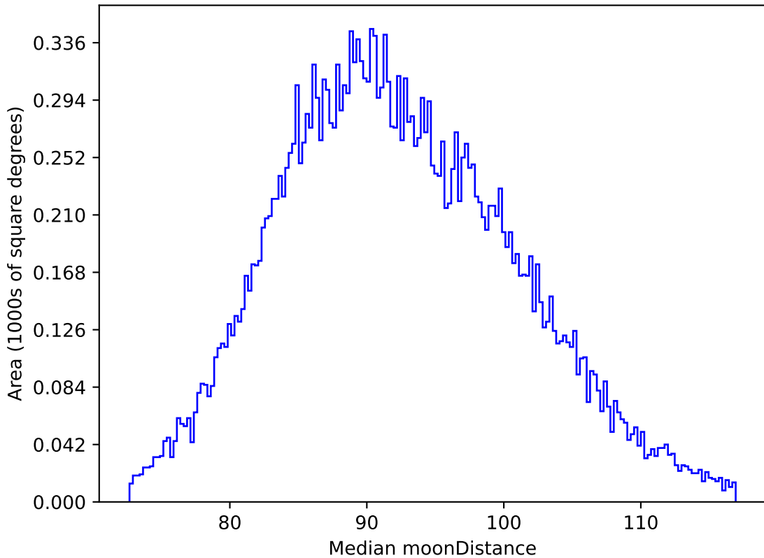
ddf_acor_sf15_lsf40_lsr10_v3.4_10yrs All sky i band: Median moonDistance
