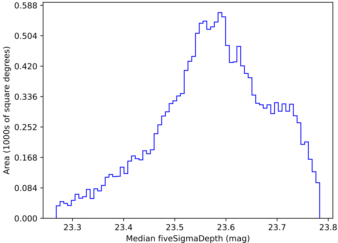
ddf_acor_sf15_lsf40_lsr10_v3.4_10yrs WFD i band: Median fiveSigmaDepth
