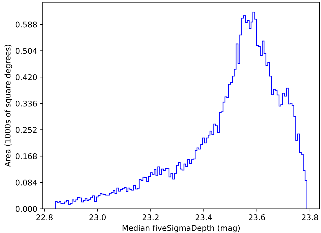
ddf_acor_sf15_lsf40_lsr10_v3.4_10yrs All sky i band: Median fiveSigmaDepth
