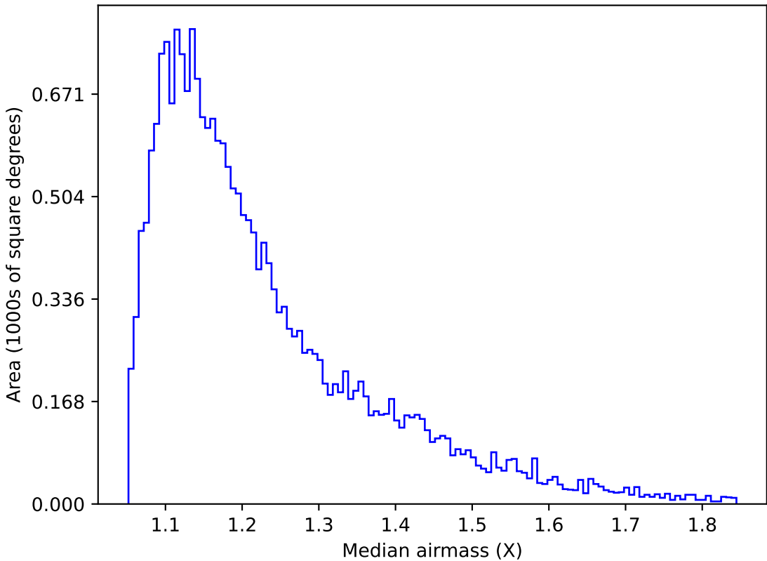
ddf_acor_sf15_lsf40_lsr10_v3.4_10yrs Yr 1 u band: Median airmass
