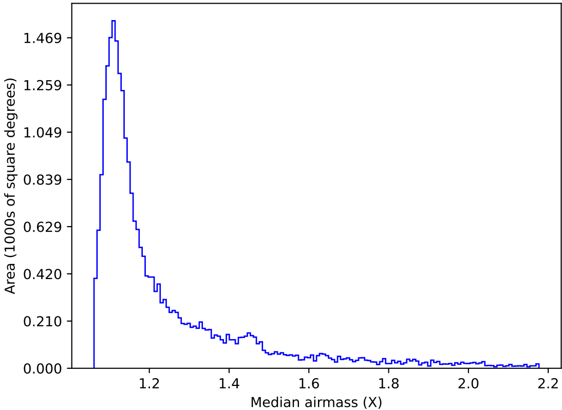
ddf_acor_sf15_lsf40_lsr10_v3.4_10yrs Yr 1 i band: Median airmass
