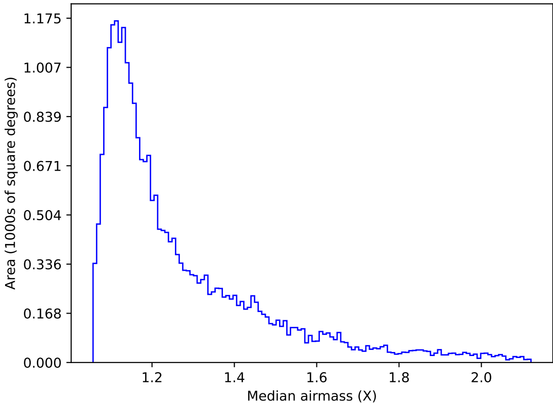
ddf_acor_sf15_lsf40_lsr10_v3.4_10yrs Yr 1 g band: Median airmass
