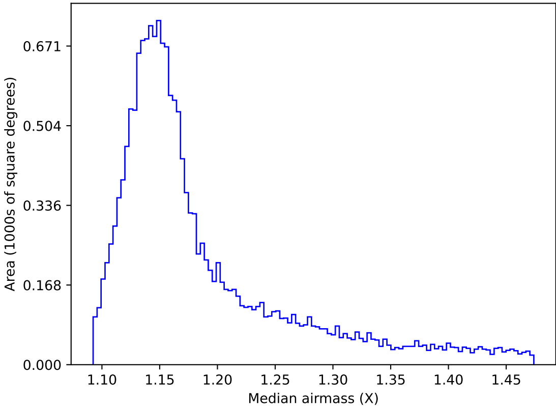
ddf_acor_sf15_lsf40_lsr10_v3.4_10yrs WFD y band: Median airmass
