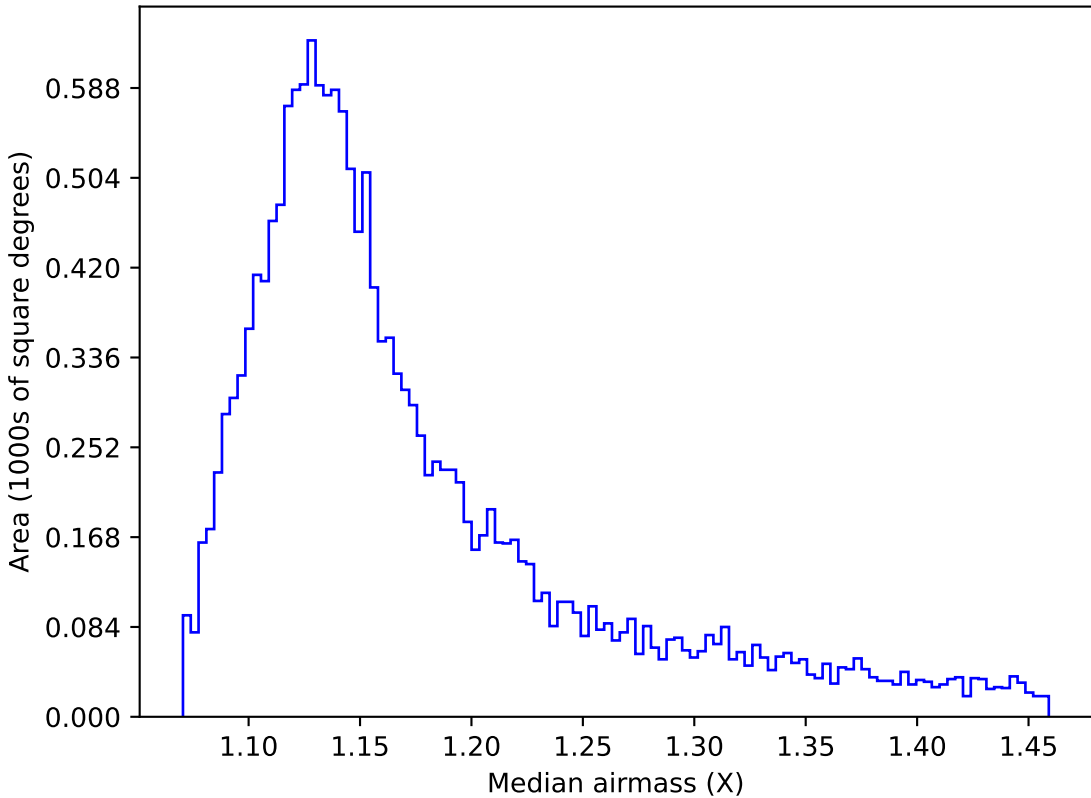
ddf_acor_sf15_lsf40_lsr10_v3.4_10yrs WFD u band: Median airmass
