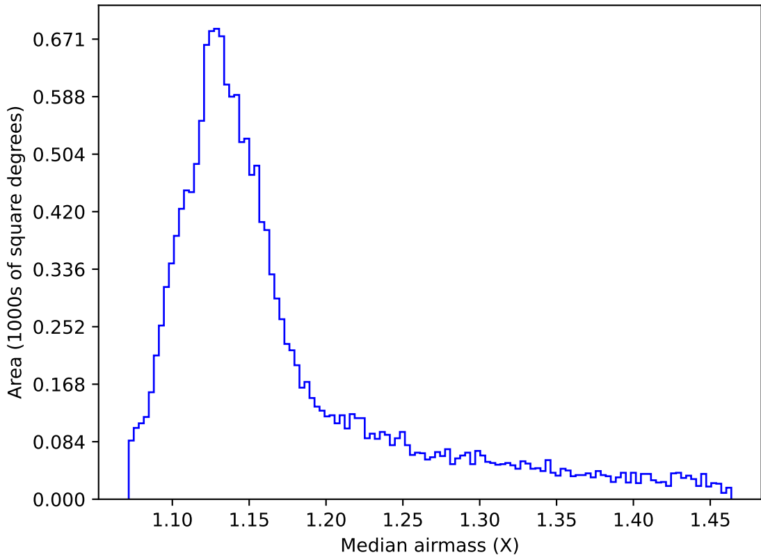
ddf_acor_sf15_lsf40_lsr10_v3.4_10yrs WFD r band: Median airmass
