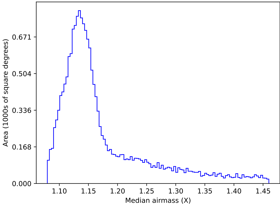
ddf_acor_sf15_lsf40_lsr10_v3.4_10yrs WFD i band: Median airmass
