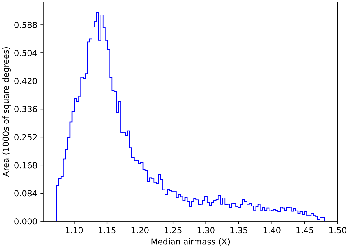
ddf_acor_sf15_lsf40_lsr10_v3.4_10yrs WFD g band: Median airmass
