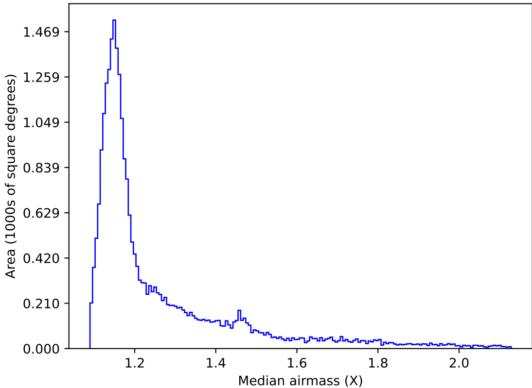
ddf_acor_sf15_lsf40_lsr10_v3.4_10yrs All sky z band: Median airmass
