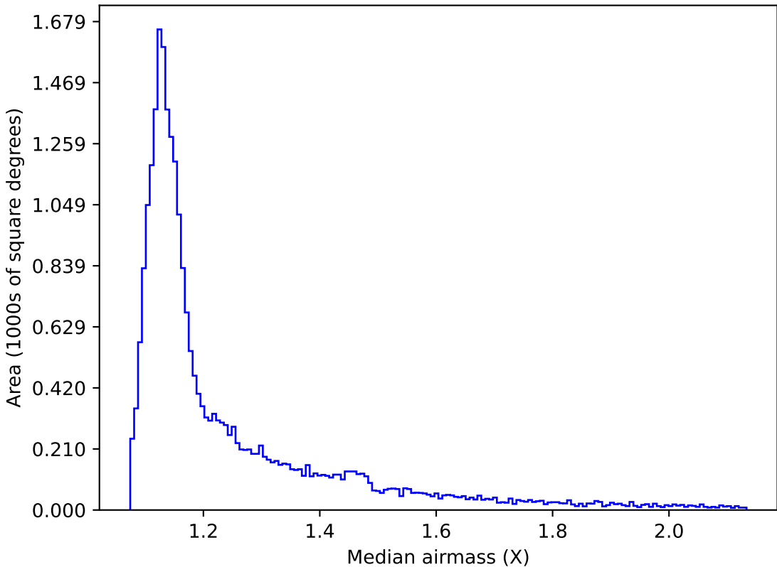
ddf_acor_sf15_lsf40_lsr10_v3.4_10yrs All sky r band: Median airmass
