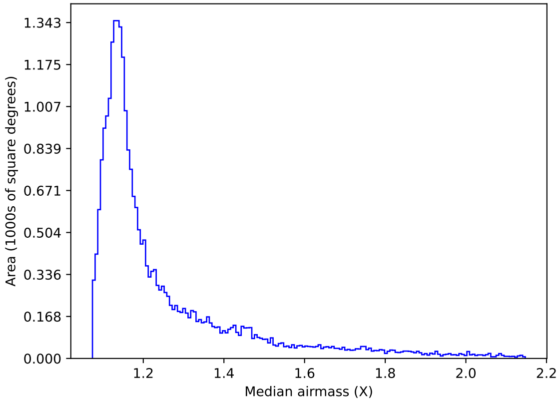
ddf_acor_sf15_lsf40_lsr10_v3.4_10yrs All sky g band: Median airmass
