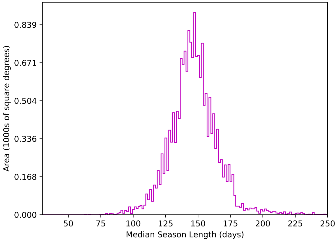
ddf_acor_sf15_lsf40_lsr10_v3.4_10yrs WFD z band: Median Season Length
