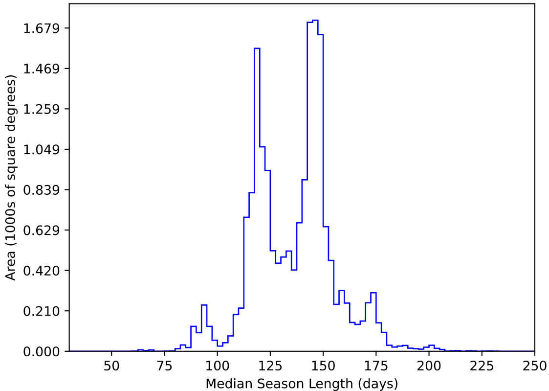
ddf_acor_sf15_lsf40_lsr10_v3.4_10yrs WFD y band: Median Season Length
