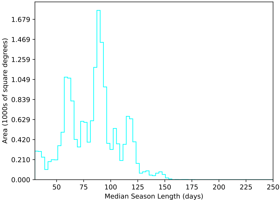
ddf_acor_sf15_lsf40_lsr10_v3.4_10yrs WFD u band: Median Season Length
