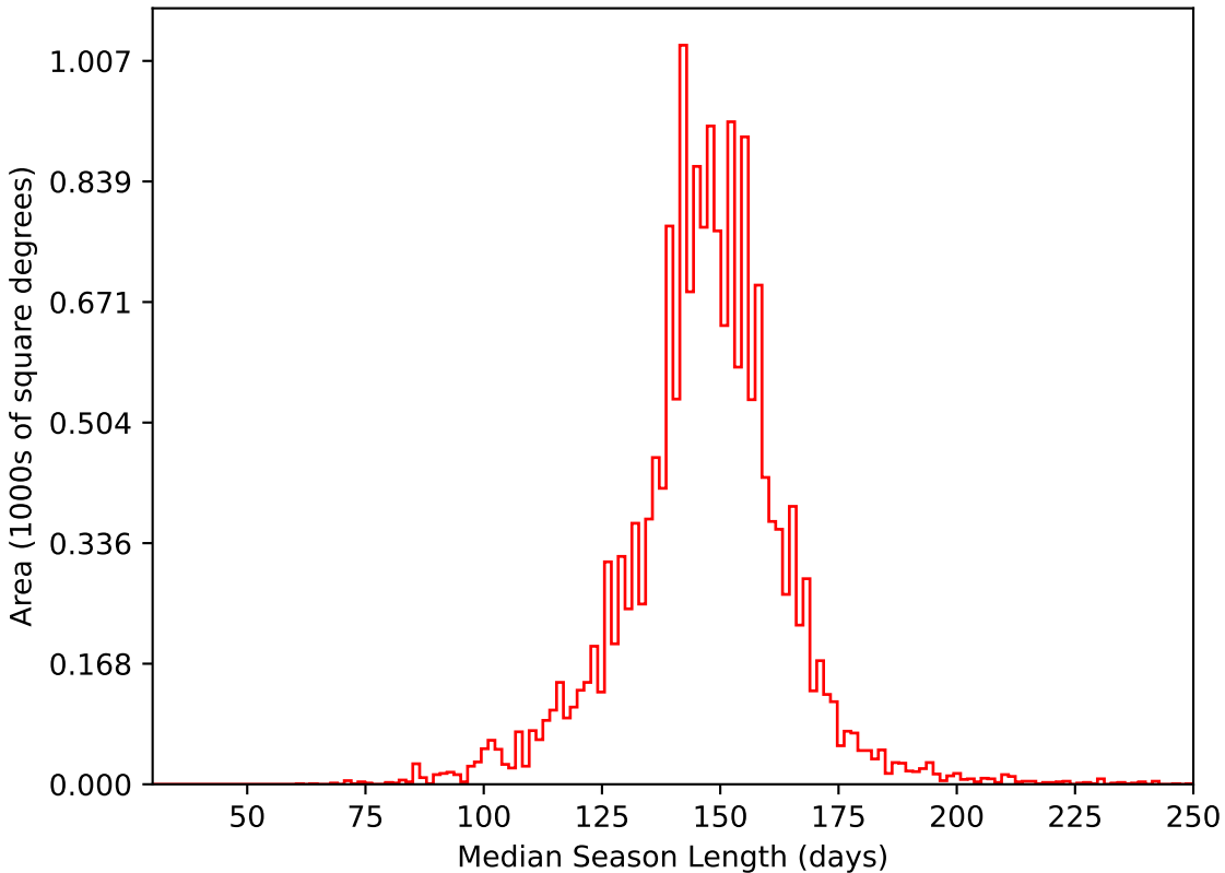
ddf_acor_sf15_lsf40_lsr10_v3.4_10yrs WFD i band: Median Season Length
