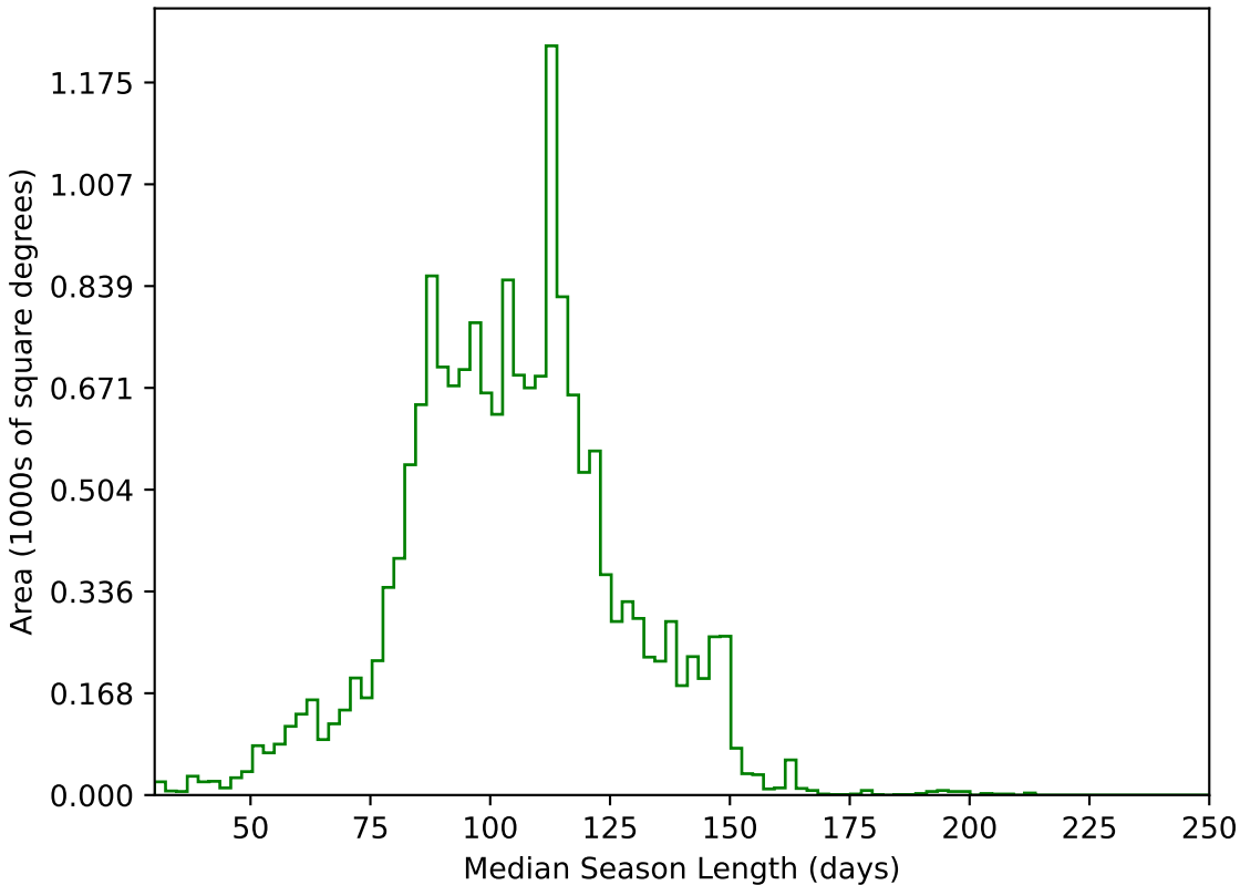
ddf_acor_sf15_lsf40_lsr10_v3.4_10yrs WFD g band: Median Season Length
