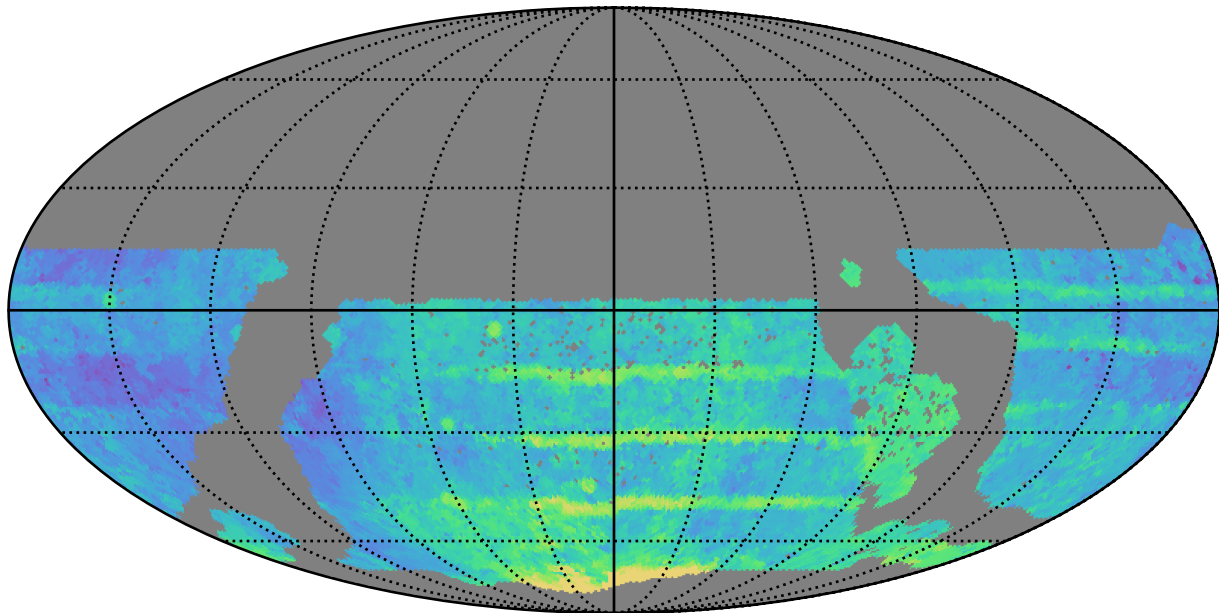
ddf_acor_sf15_lsf40_lsr10_v3.4_10yrs WFD all bands: Median Season Length
