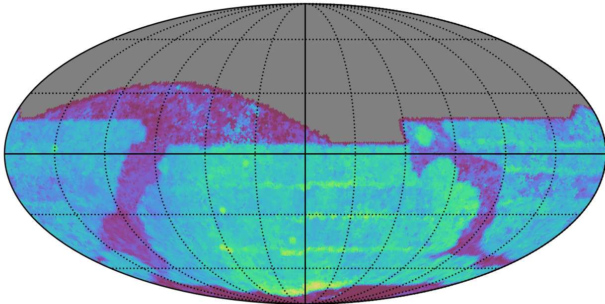
ddf_acor_sf15_lsf40_lsr10_v3.4_10yrs All sky z band: Median Season Length
