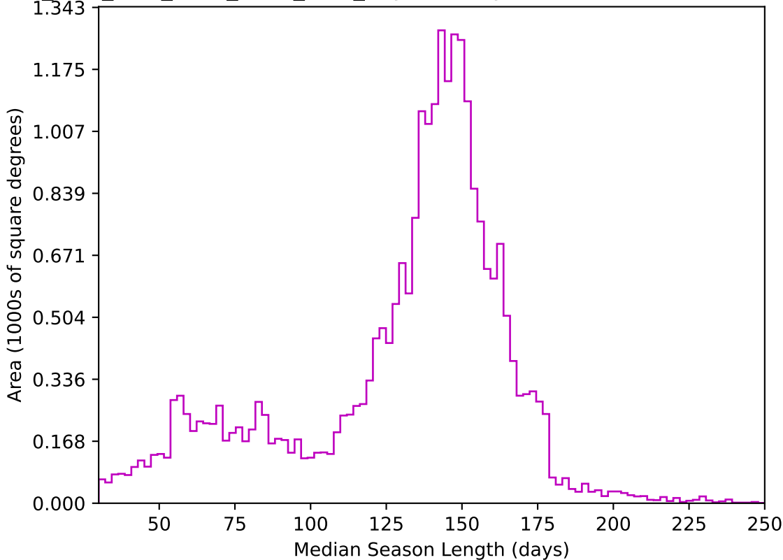
ddf_acor_sf15_lsf40_lsr10_v3.4_10yrs All sky z band: Median Season Length
