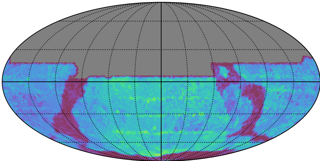
ddf_acor_sf15_lsf40_lsr10_v3.4_10yrs All sky y band: Median Season Length
