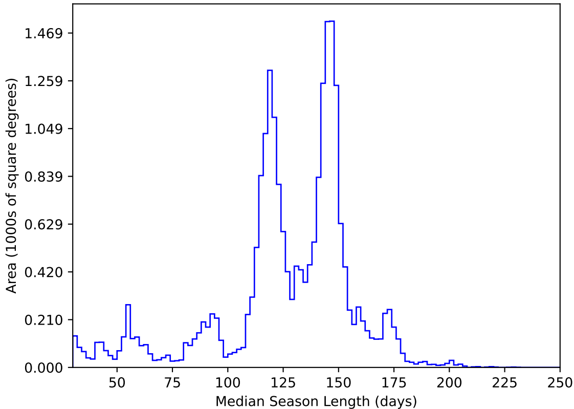
ddf_acor_sf15_lsf40_lsr10_v3.4_10yrs All sky y band: Median Season Length
