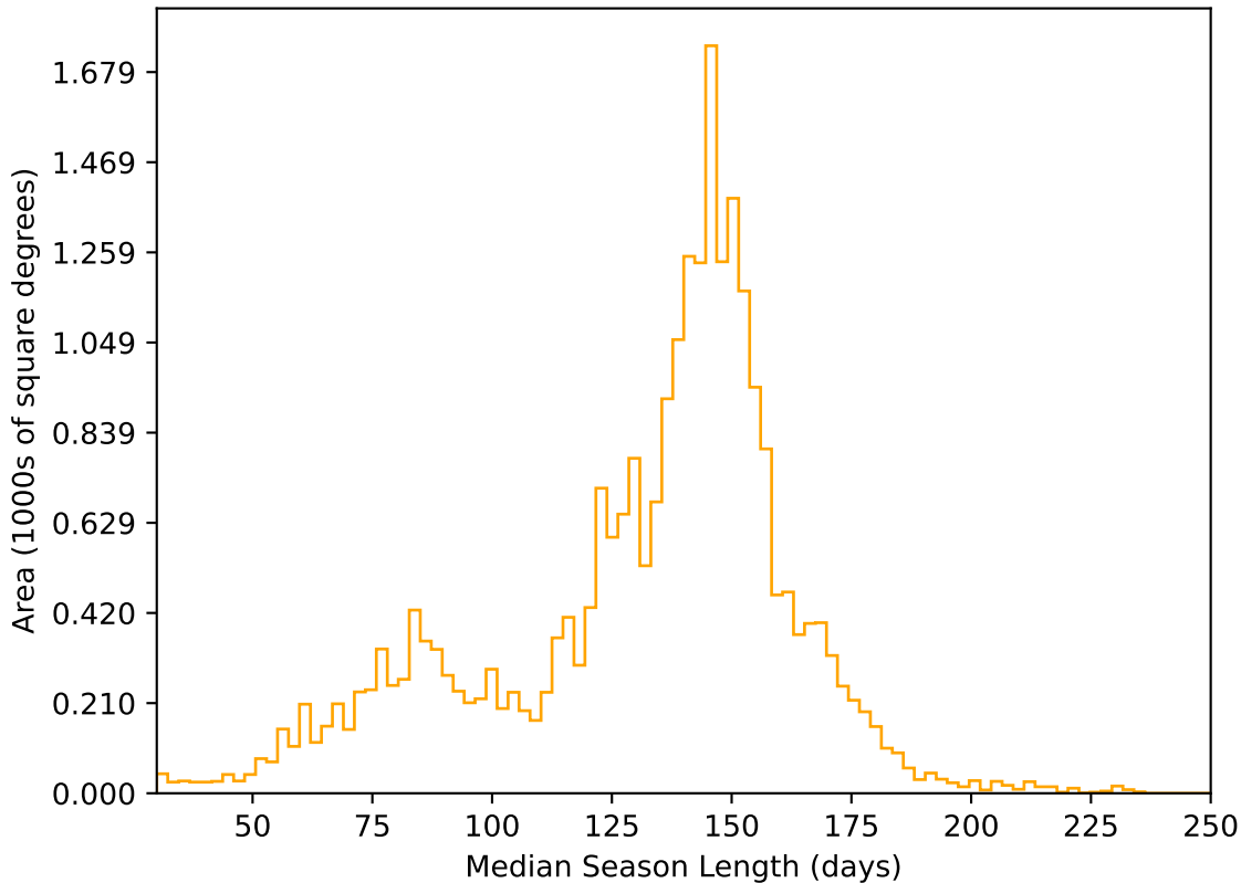
ddf_acor_sf15_lsf40_lsr10_v3.4_10yrs All sky r band: Median Season Length
