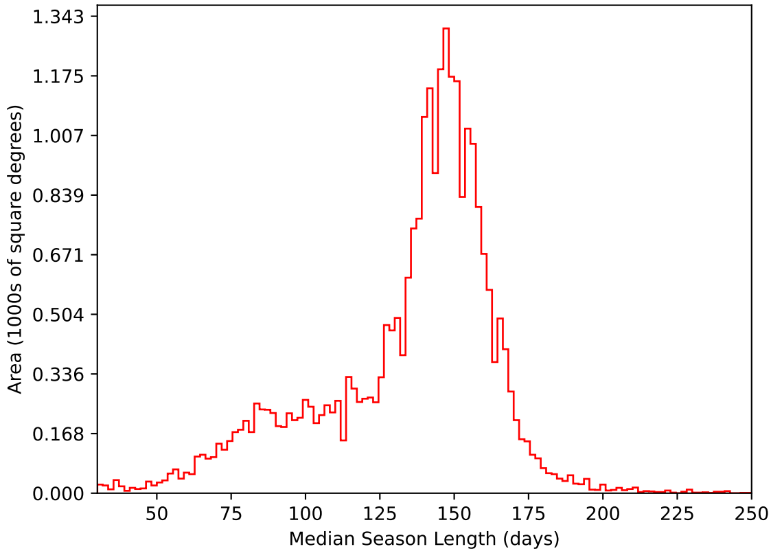
ddf_acor_sf15_lsf40_lsr10_v3.4_10yrs All sky i band: Median Season Length
