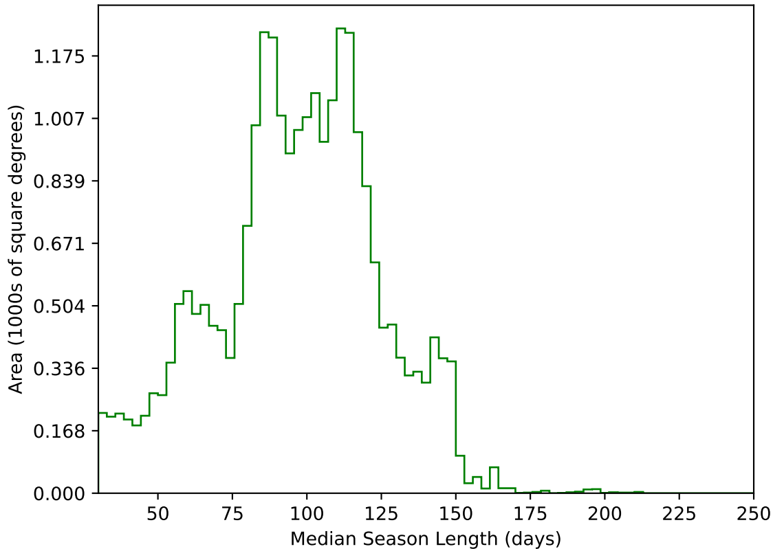
ddf_acor_sf15_lsf40_lsr10_v3.4_10yrs All sky g band: Median Season Length
