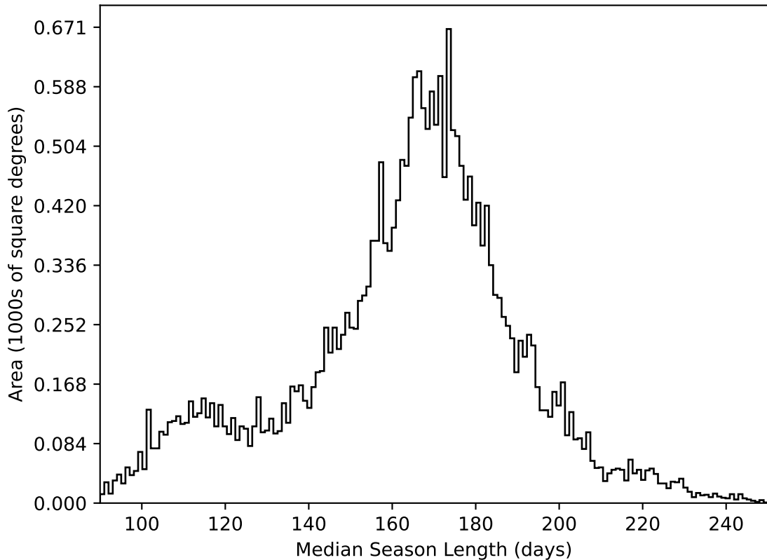
ddf_acor_sf15_lsf40_lsr10_v3.4_10yrs All sky all bands: Median Season Length
