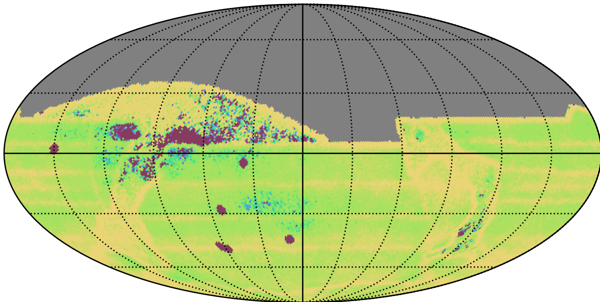
ddf_acor_sf15_lsf40_lsr10_v3.4_10yrs All sky: Median Intra-Night Gap
