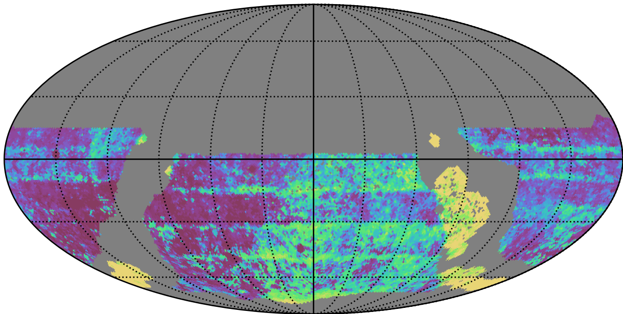
ddf_acor_sf15_lsf40_lsr10_v3.4_10yrs WFD y band: Median Inter-Night Gap
