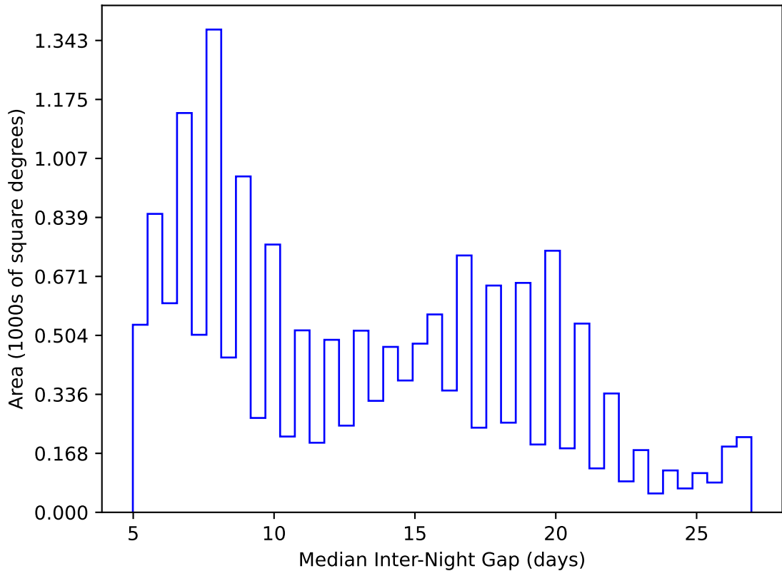
ddf_acor_sf15_lsf40_lsr10_v3.4_10yrs WFD y band: Median Inter-Night Gap
