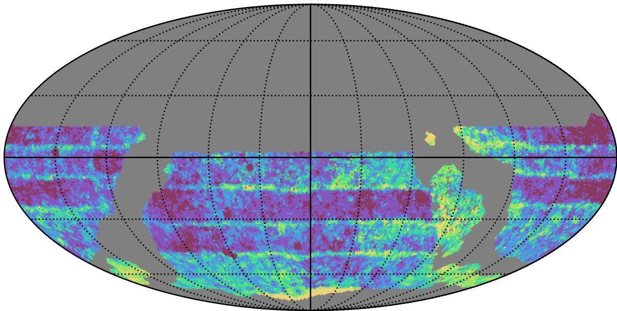
ddf_acor_sf15_lsf40_lsr10_v3.4_10yrs WFD r band: Median Inter-Night Gap
