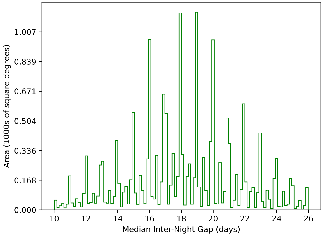
ddf_acor_sf15_lsf40_lsr10_v3.4_10yrs WFD g band: Median Inter-Night Gap
