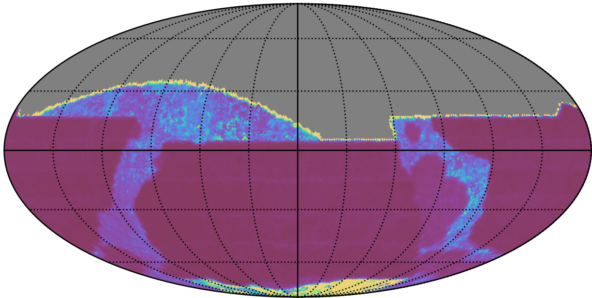
ddf_acor_sf15_lsf40_lsr10_v3.4_10yrs All sky z band: Median Inter-Night Gap
