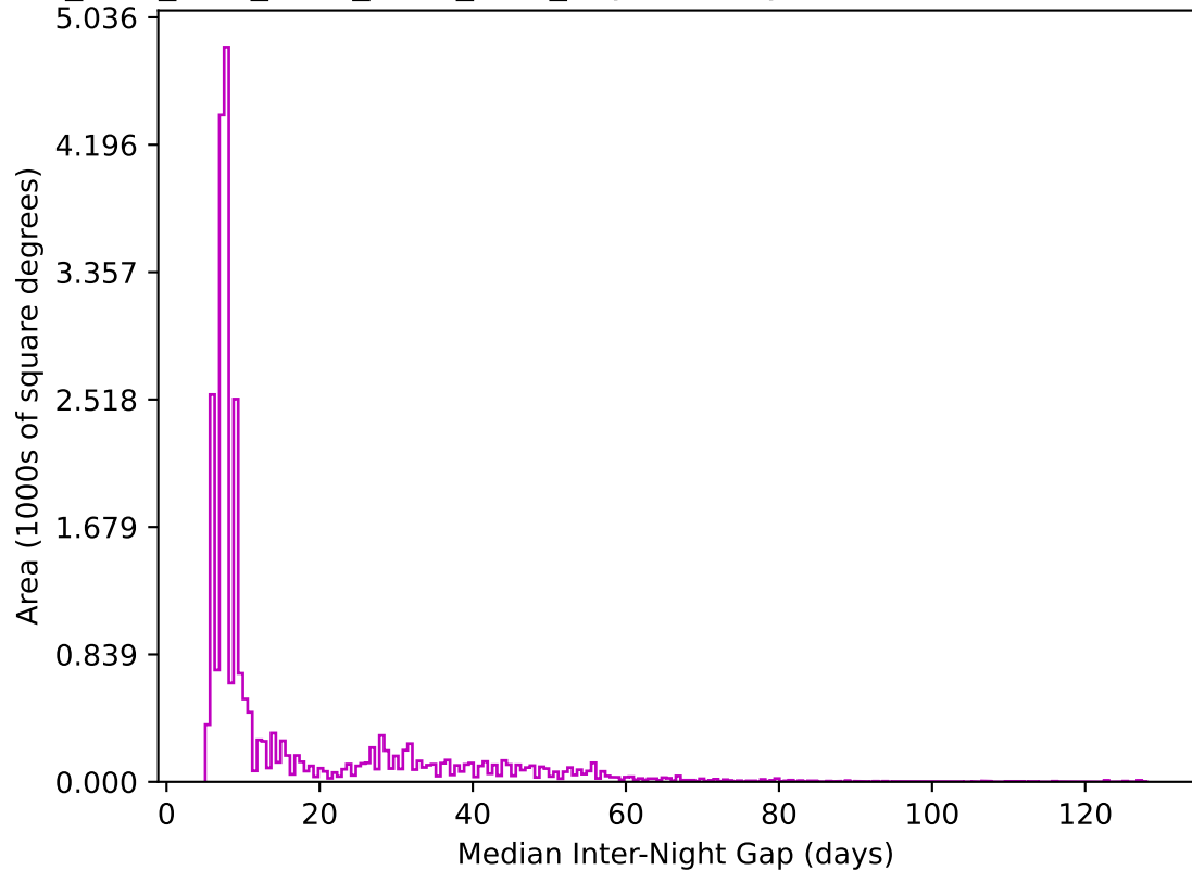
ddf_acor_sf15_lsf40_lsr10_v3.4_10yrs All sky z band: Median Inter-Night Gap
