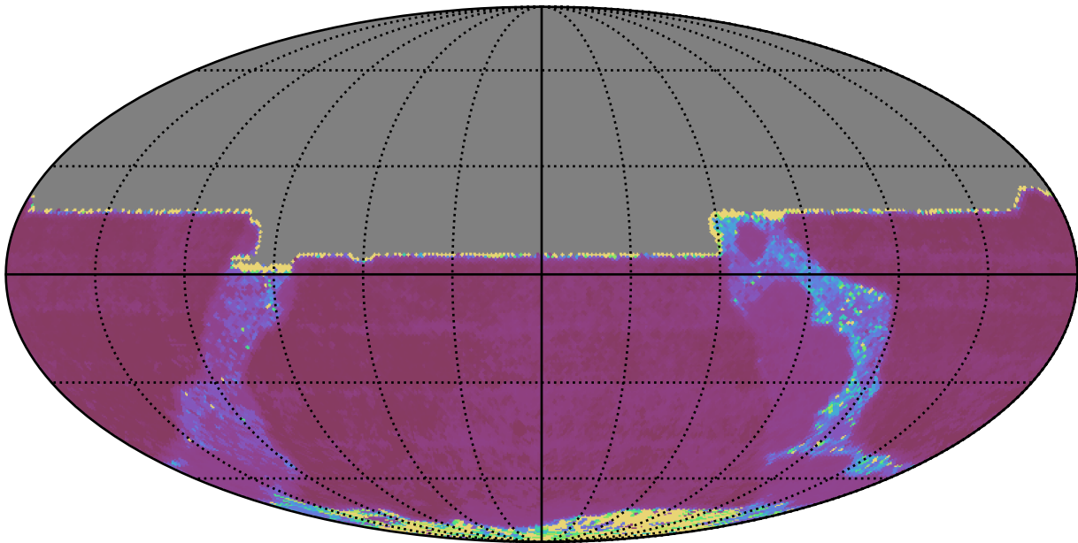
ddf_acor_sf15_lsf40_lsr10_v3.4_10yrs All sky y band: Median Inter-Night Gap
