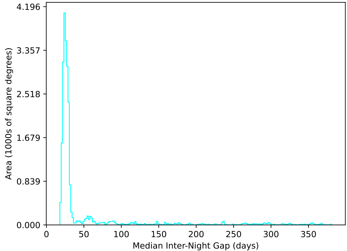
ddf_acor_sf15_lsf40_lsr10_v3.4_10yrs All sky u band: Median Inter-Night Gap
