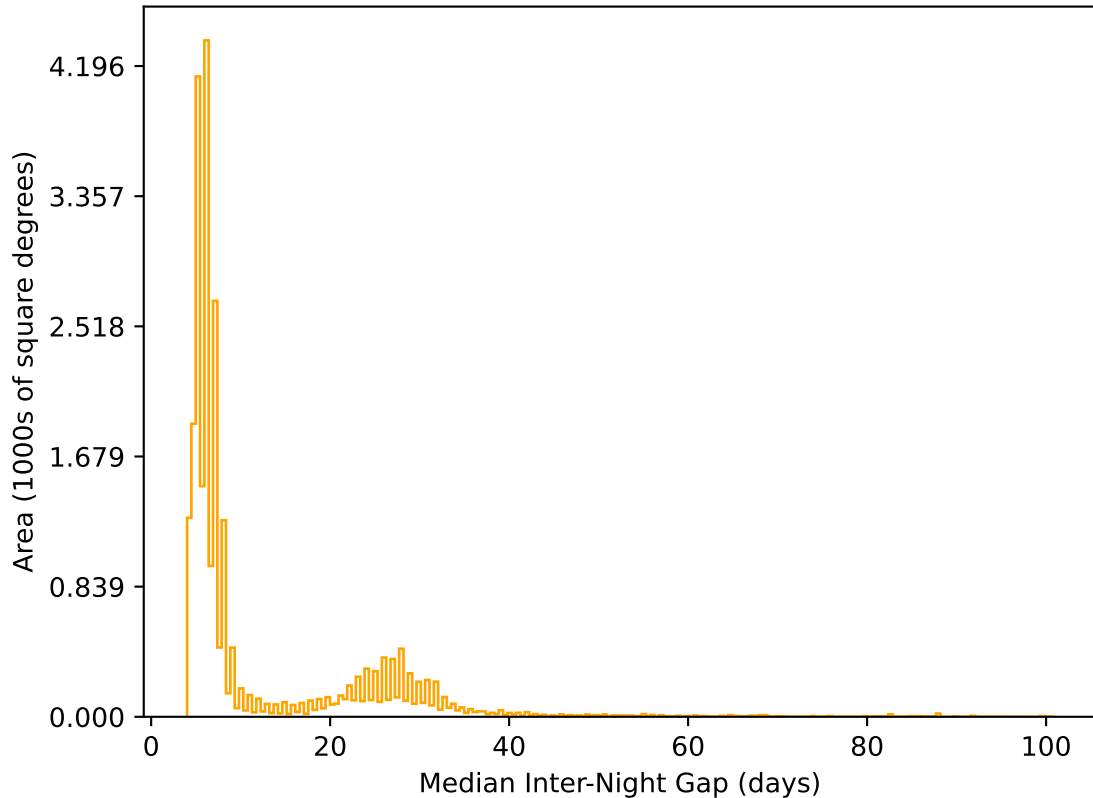
ddf_acor_sf15_lsf40_lsr10_v3.4_10yrs All sky r band: Median Inter-Night Gap
