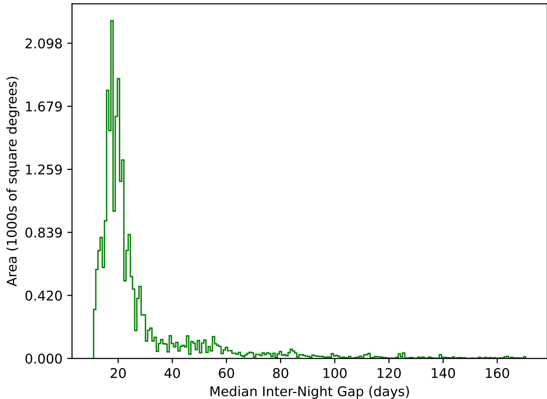
ddf_acor_sf15_lsf40_lsr10_v3.4_10yrs All sky g band: Median Inter-Night Gap
