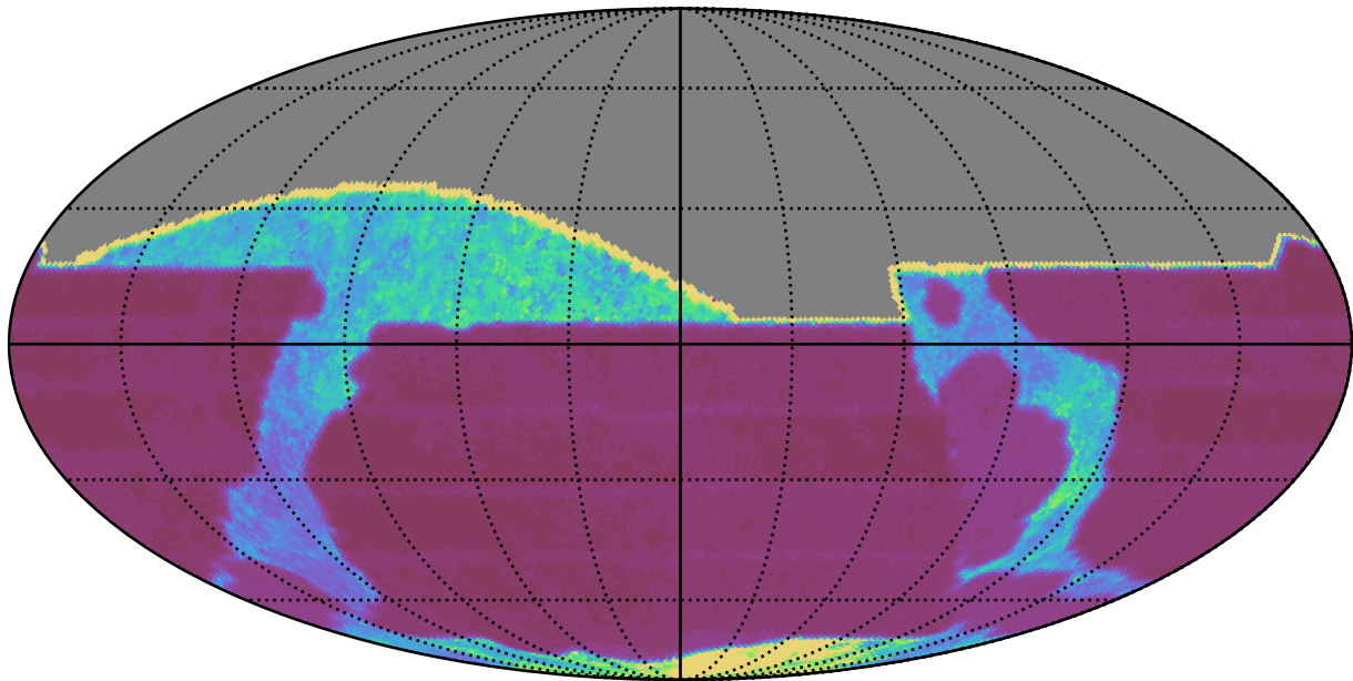
ddf_acor_sf15_lsf40_lsr10_v3.4_10yrs All sky all bands: Median Inter-Night Gap
