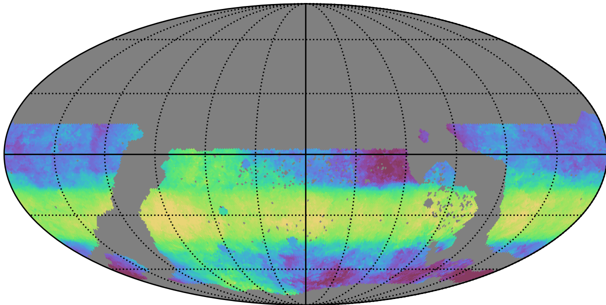
ddf_acor_sf15_lsf40_lsr10_v3.4_10yrs WFD z band: Median HA
