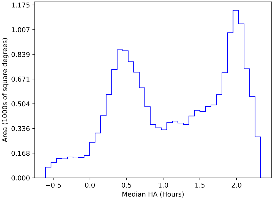
ddf_acor_sf15_lsf40_lsr10_v3.4_10yrs WFD z band: Median HA
