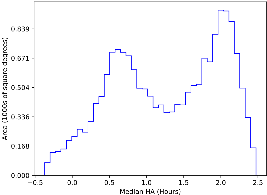
ddf_acor_sf15_lsf40_lsr10_v3.4_10yrs WFD y band: Median HA
