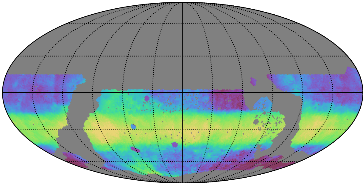
ddf_acor_sf15_lsf40_lsr10_v3.4_10yrs WFD i band: Median HA
