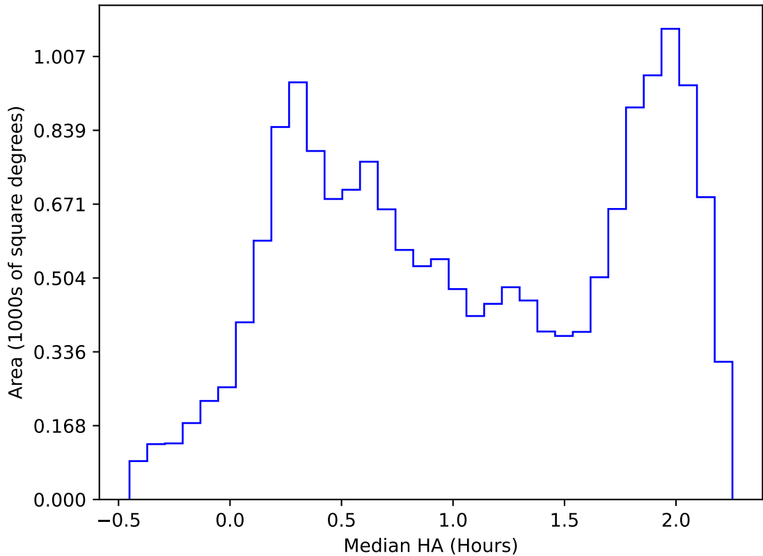
ddf_acor_sf15_lsf40_lsr10_v3.4_10yrs WFD i band: Median HA
