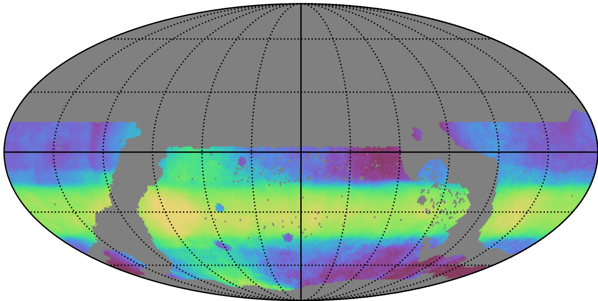
ddf_acor_sf15_lsf40_lsr10_v3.4_10yrs WFD all bands: Median HA
