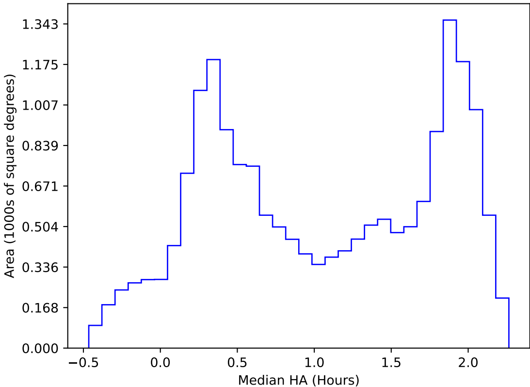
ddf_acor_sf15_lsf40_lsr10_v3.4_10yrs WFD all bands: Median HA
