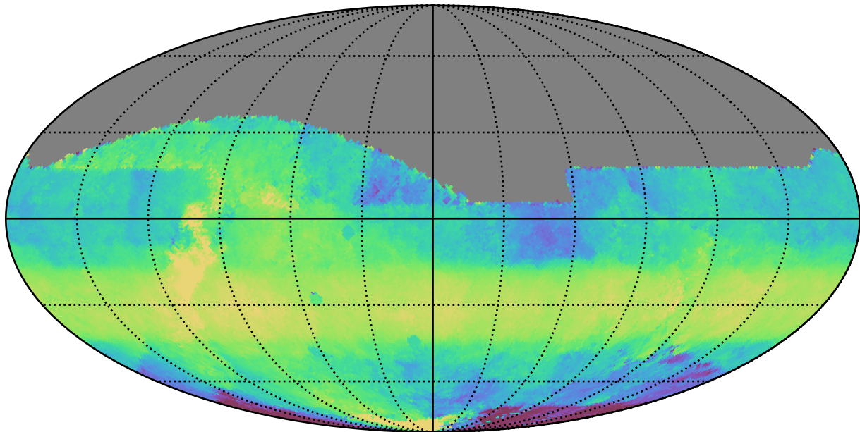
ddf_acor_sf15_lsf40_lsr10_v3.4_10yrs All sky z band: Median HA
